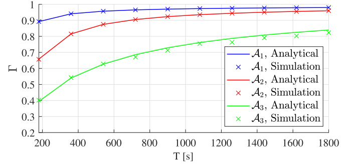
Fig. 13. Gain of the aggregation protocol, analytical expression, and simulation.
