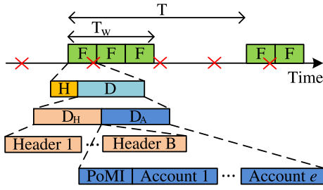
Fig. 5. Periodic release of information. Red crosses represent block generations. In the first release, there are two retransmissions of the frame ( F ), due to failure, in the second release, only one retransmission.
